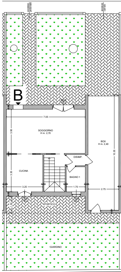
PIANO TERRA
