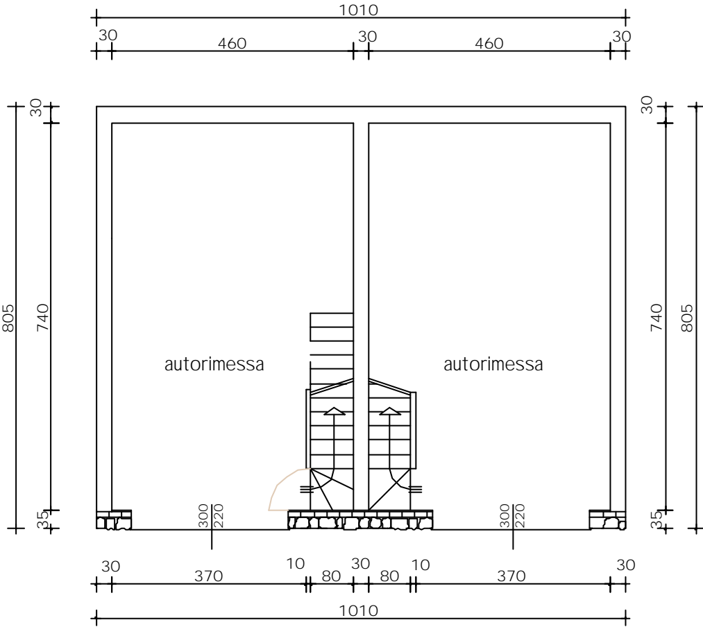
PIANO INTERRATO
